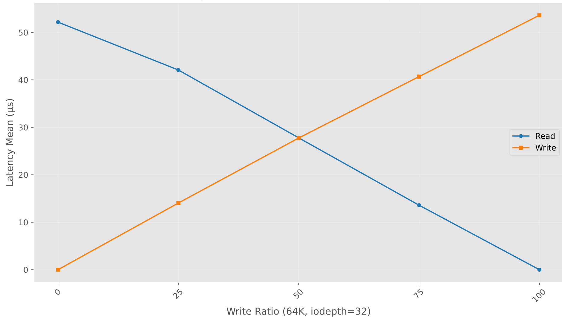
Latency Mean vs Write Ratio (64K, iodepth=32)
